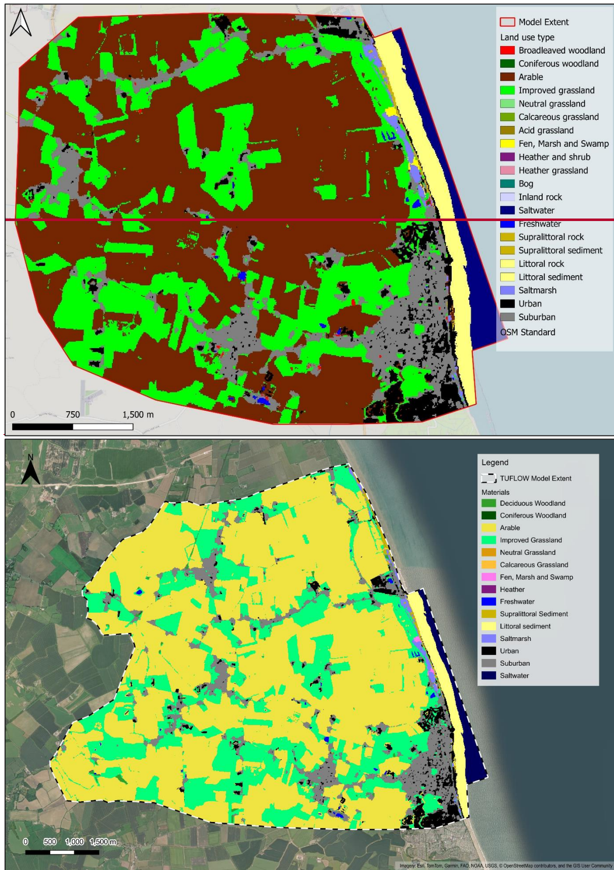
Figure 2-45: Hydraulic Model Material Roughness
