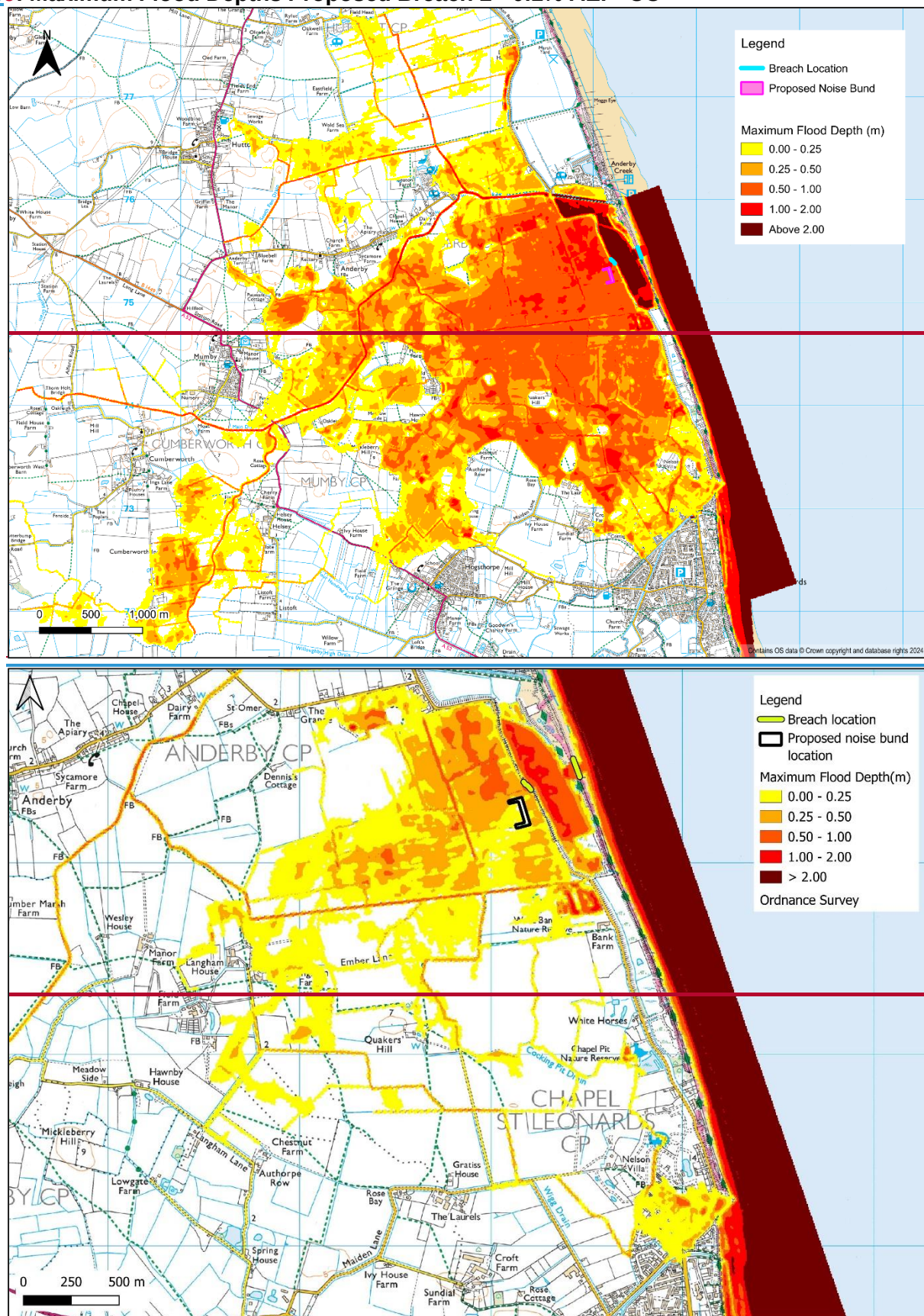
Figure 3-59: Maximum Flood Depths Proposed Breach 2 - 0.1% AEP+CC
