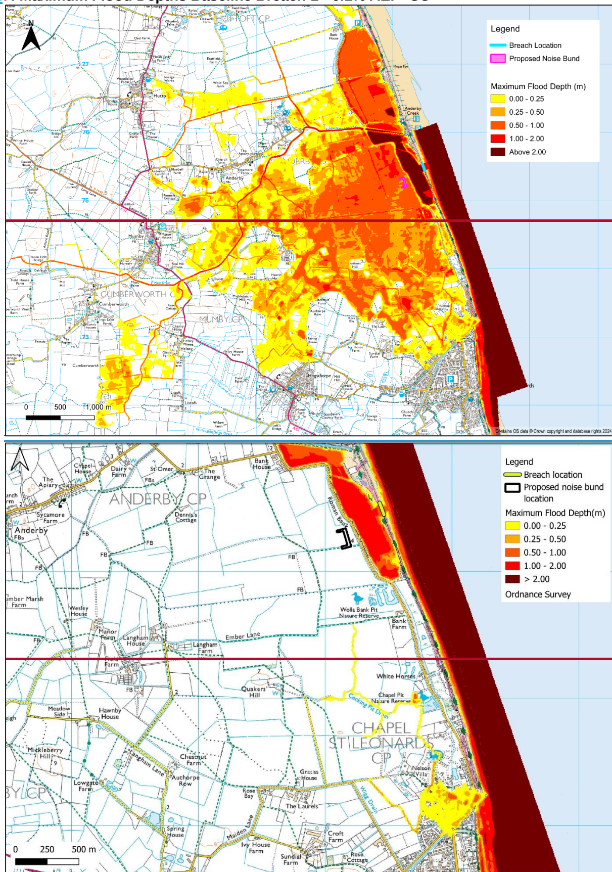
Figure 3-27: Maximum Flood Depths Baseline Breach 1 - 0.1% AEP+CC
