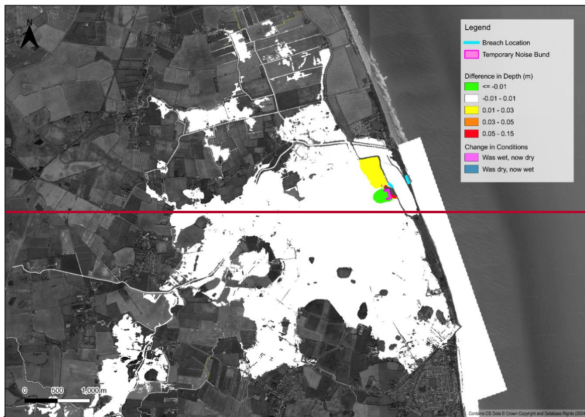
Figure 3-710: Flood Depth-Level Difference Proposed vs Baseline Breach 2 - 0.1% AEP+CC
