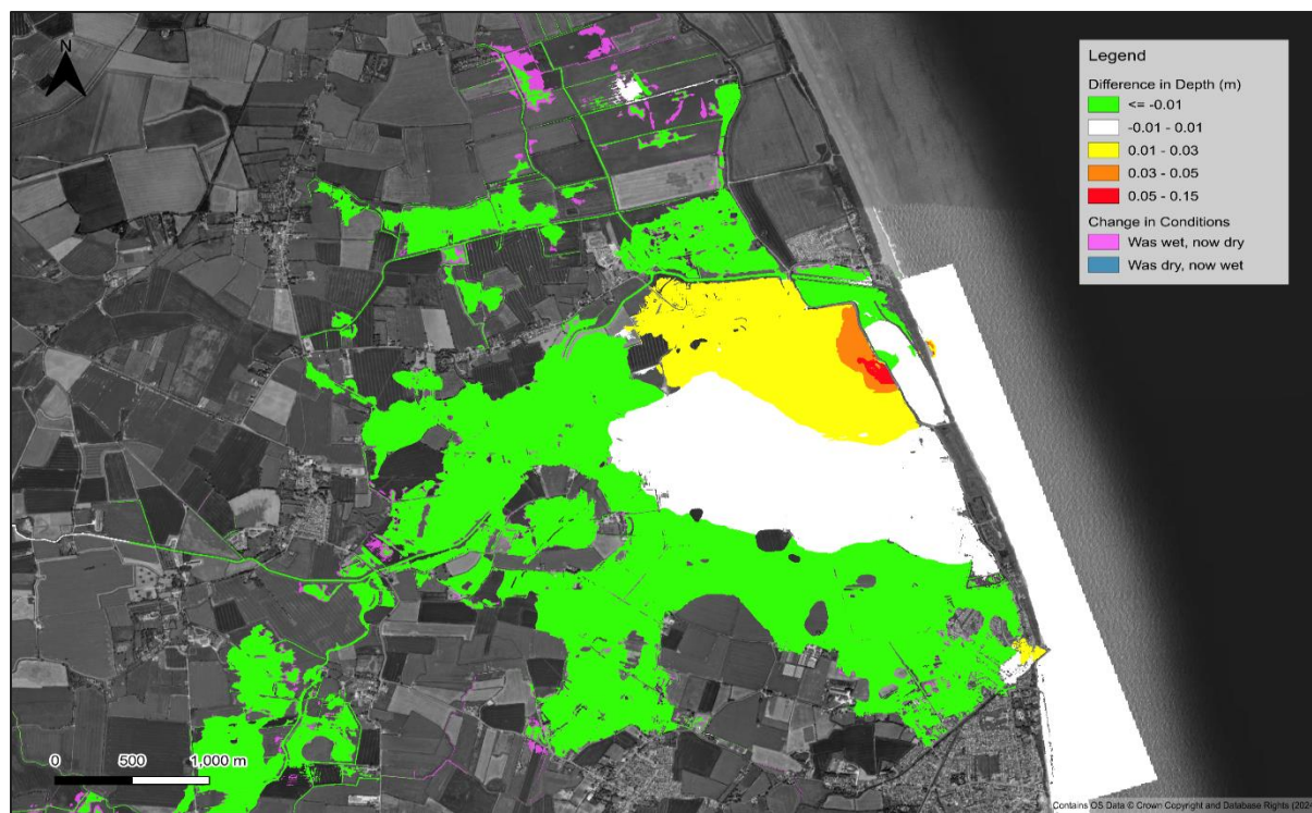
Figure 4-3: Peak Water Level Difference +20% Manning's Roughness (vs Baseline)
