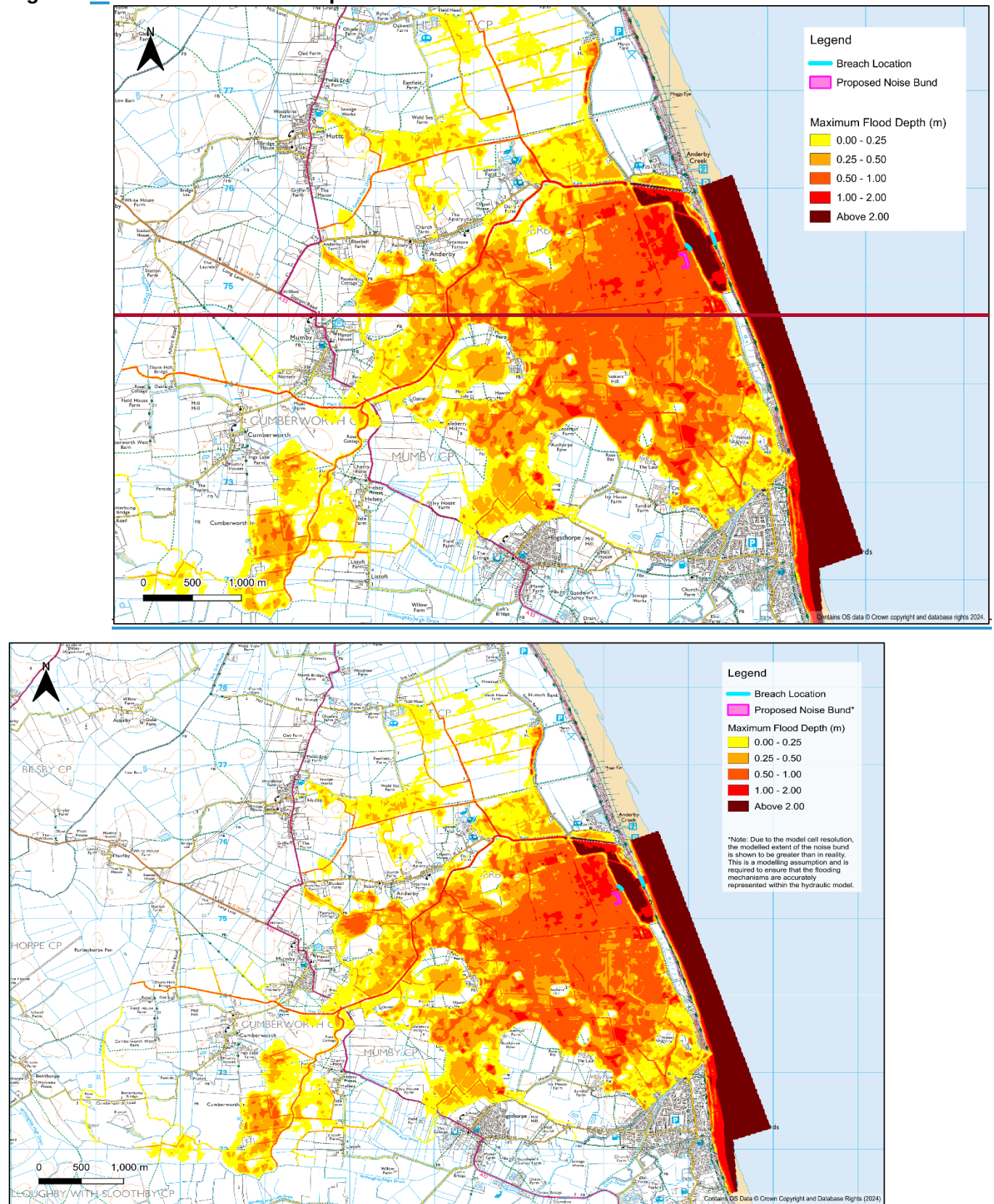
Figure 3-38: Maximum Flood Depths Baseline Breach 2 - 0.1% AEP+CC
