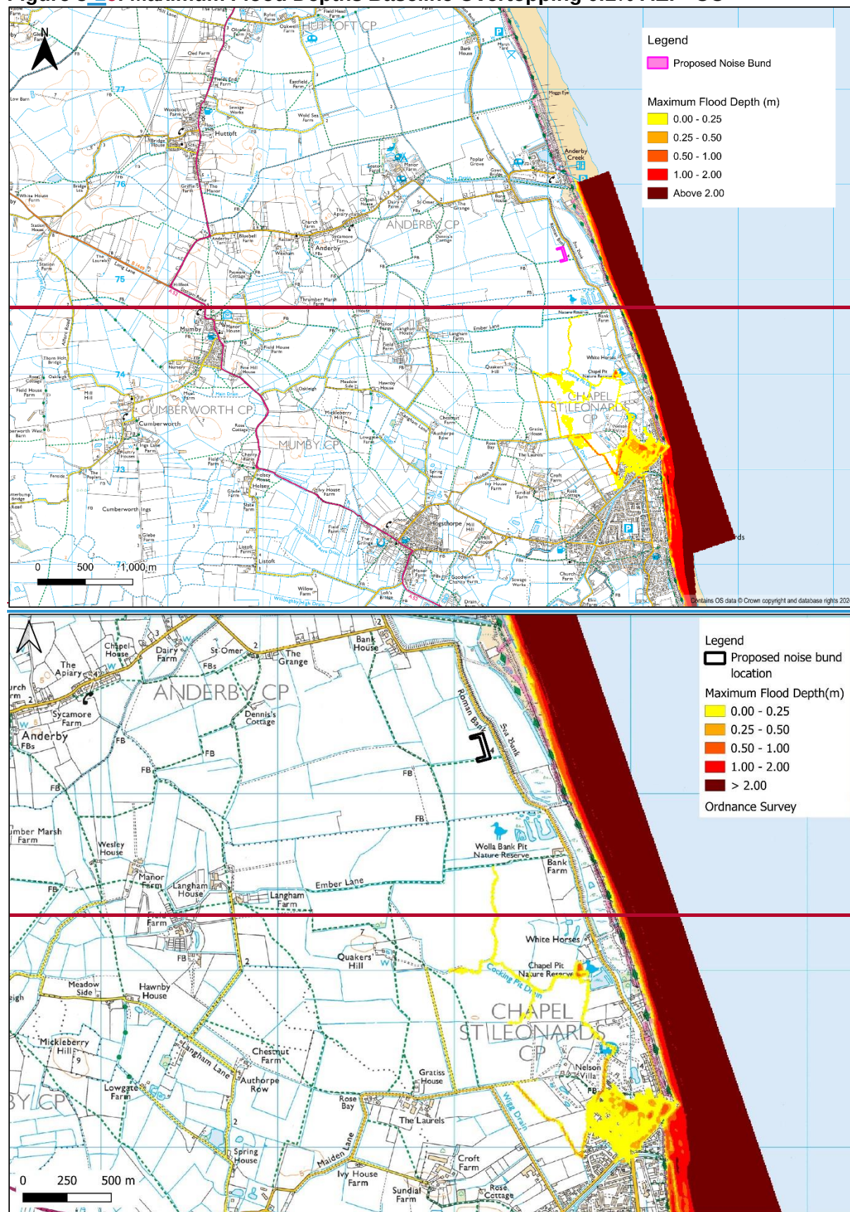
Figure 3-16: Maximum Flood Depths Baseline Overtopping 0.1% AEP+CC
