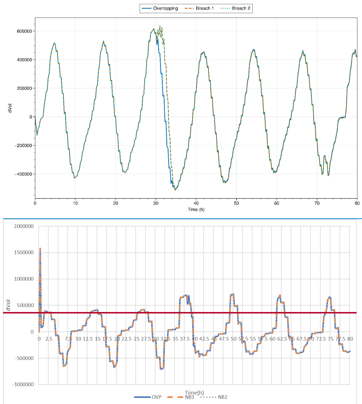
Figure 3-912: Comparison of dVol for Overtopping and Breach Scenarios
