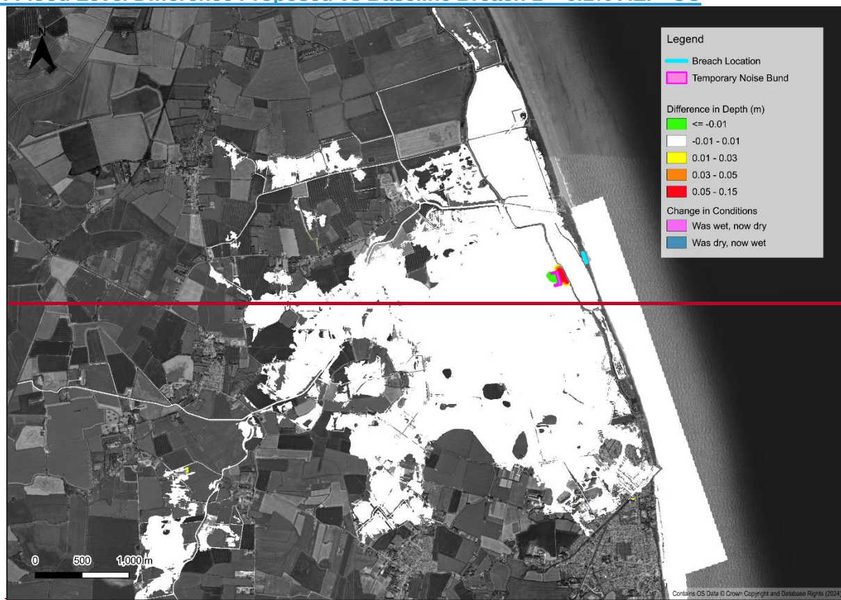
Figure 3-6: Flood Level Difference Proposed vs Baseline Breach 1 – 0.1% AEP+CC
