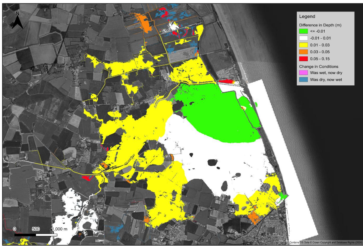
Figure 4-214: Peak Water Level Difference -20% Manning's Roughness (vs Baseline) Flood Extent of Difference Roughness Sensitivity Runs
